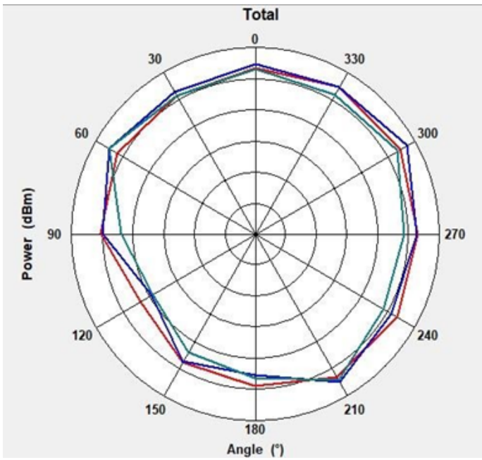
2.4 GHz Antenna Radiation Pattern
