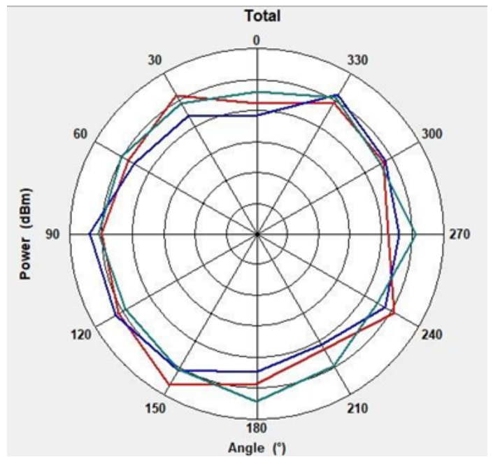
5.5 GHz Antenna Radiation Pattern
