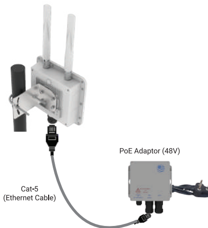
Power up using PoE Adaptor
